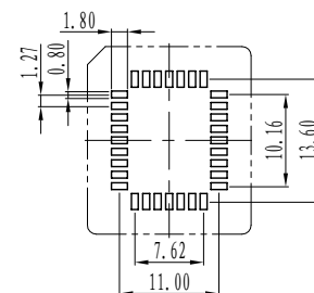
32PIN PCB LAYOUT
