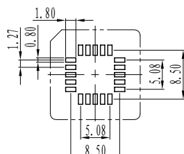
20PIN PCB LAYOUT
