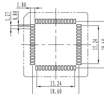
52PIN PCB LAYOUT
