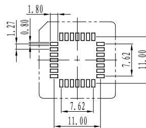
28PIN PCB LAYOUT
