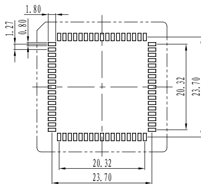
68PIN PCB LAYOUT
