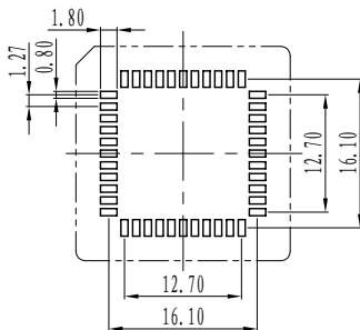
44PIN PCB LAYOUT
