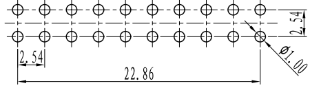
Recommended PCB LAYOUT (PCB TOLERANCE ± 0.05)
