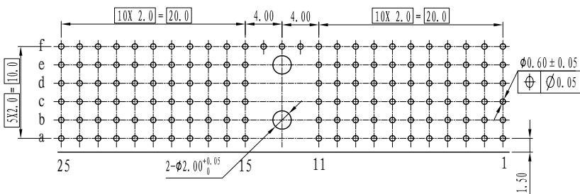
PCB LAYOUT
